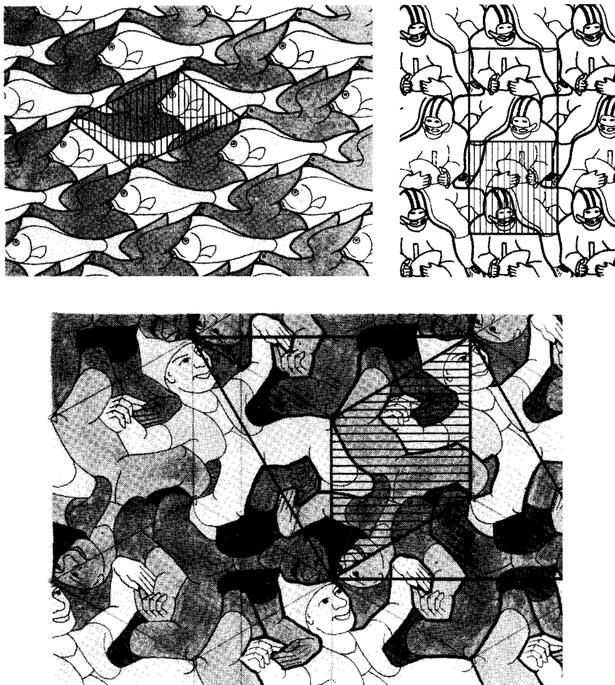
Figure 28.21 A lattice unit and generating region for the patterns in Figures 28.12, 28.13, and 28.14. Generating regions are shaded with bars.
