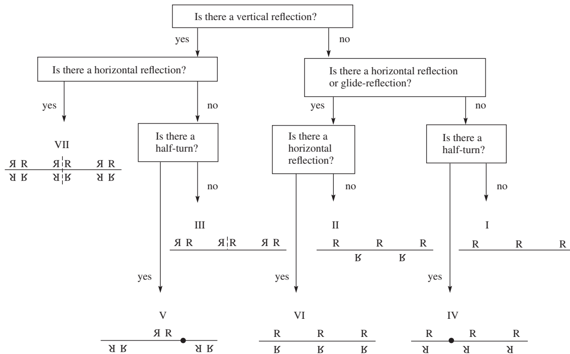
Figure 28.10 Recognition chart for frieze patterns. Adapted from [6, p. 83].
