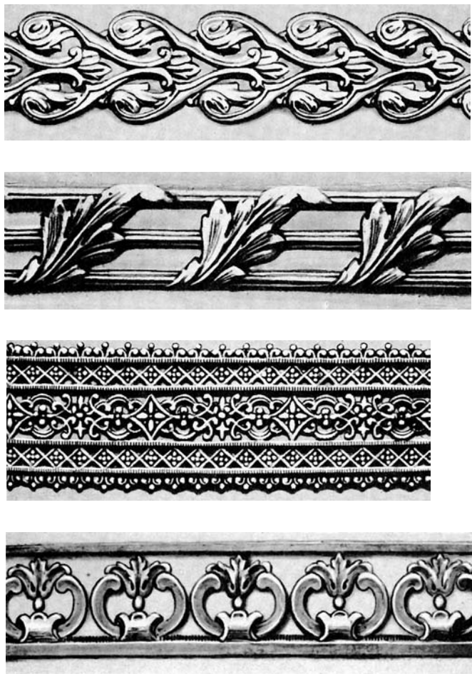
Figure 28.1 Frieze patterns
