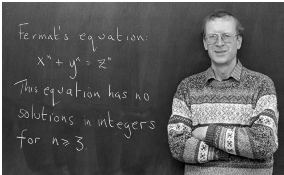
Figure 18.2 Andrew Wiles
