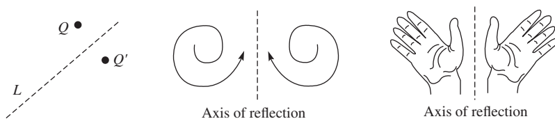
Figure 27.1 Reflected images
