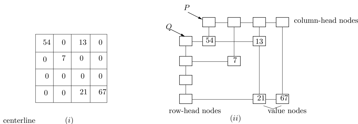
Figure 1: (ii) shows a skeleton the link based data structure for the sparse matrix shown in (i)
